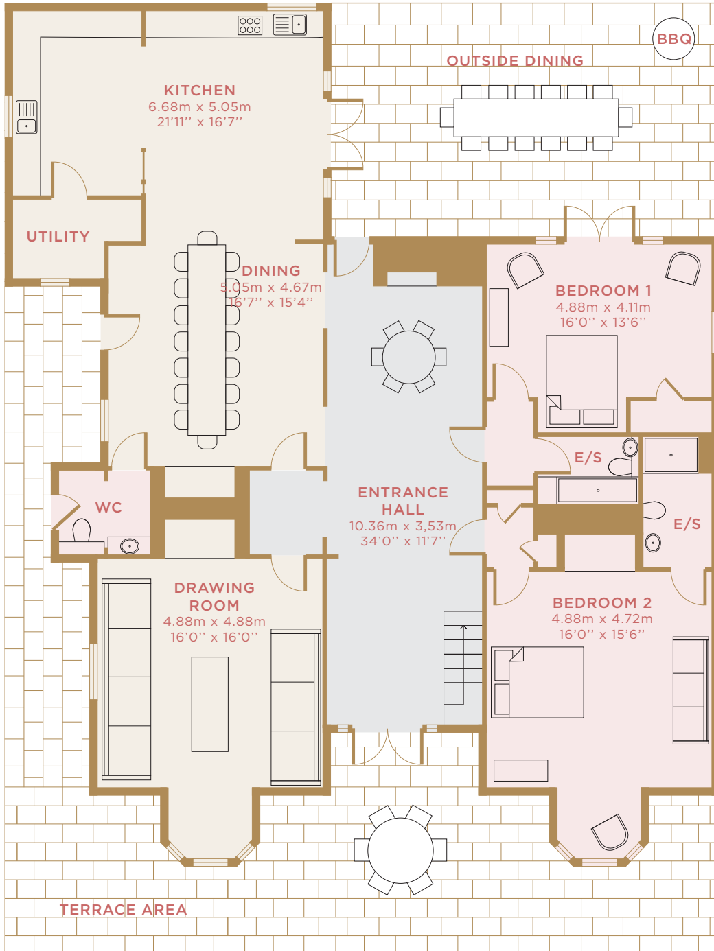
GROUND FLOOR
